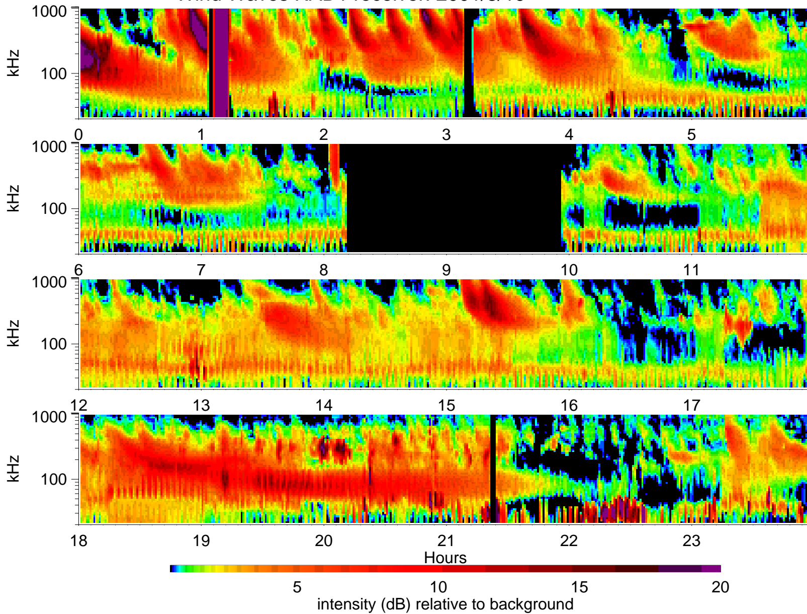
Wind Waves RAD1 receiver: 2001/3/19
