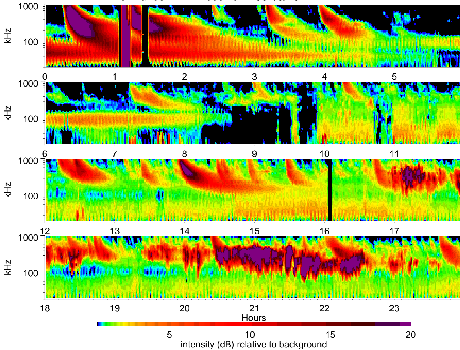
Wind Waves RAD1 receiver: 2001/3/13
