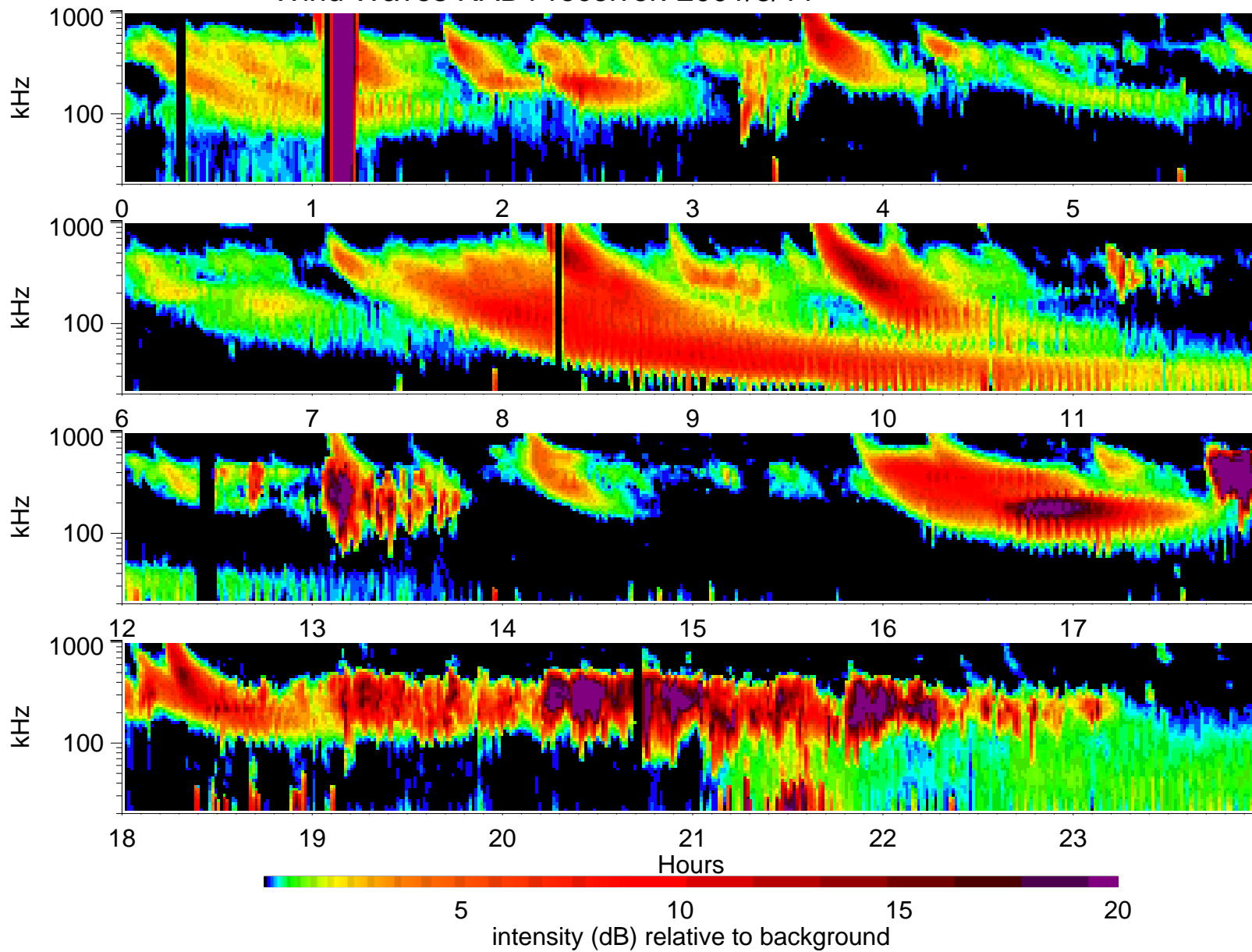
Wind Waves RAD1 receiver: 2001/3/11
