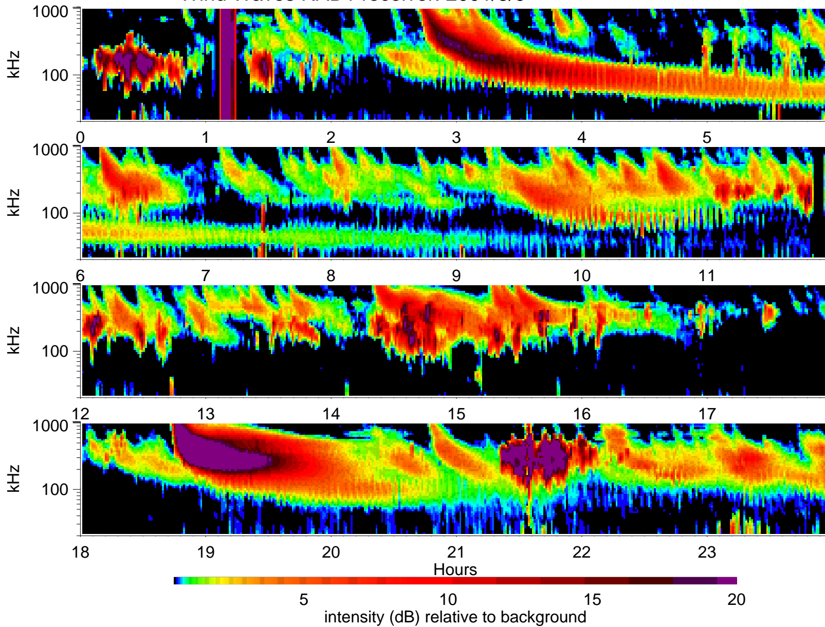
Wind Waves RAD1 receiver: 2001/3/9
