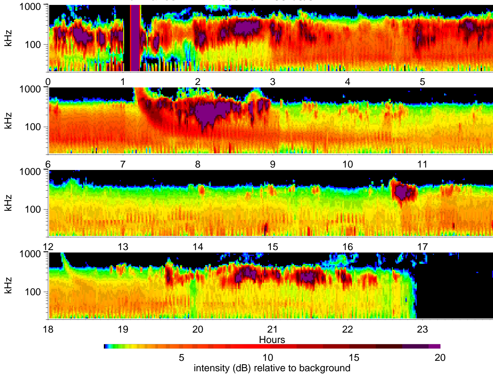
Wind Waves RAD1 receiver: 2001/3/5
