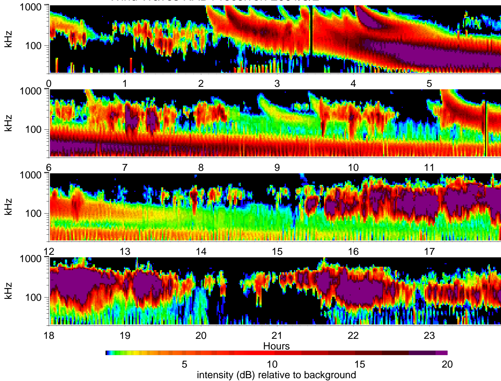
Wind Waves RAD1 receiver: 2001/3/2
