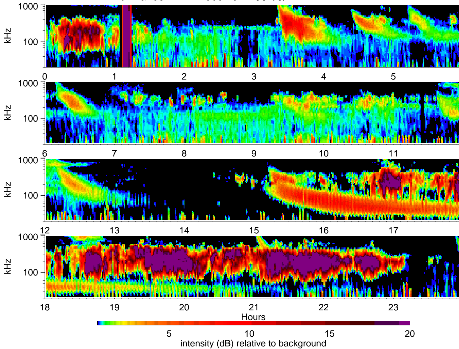
Wind Waves RAD1 receiver: 2001/3/1
