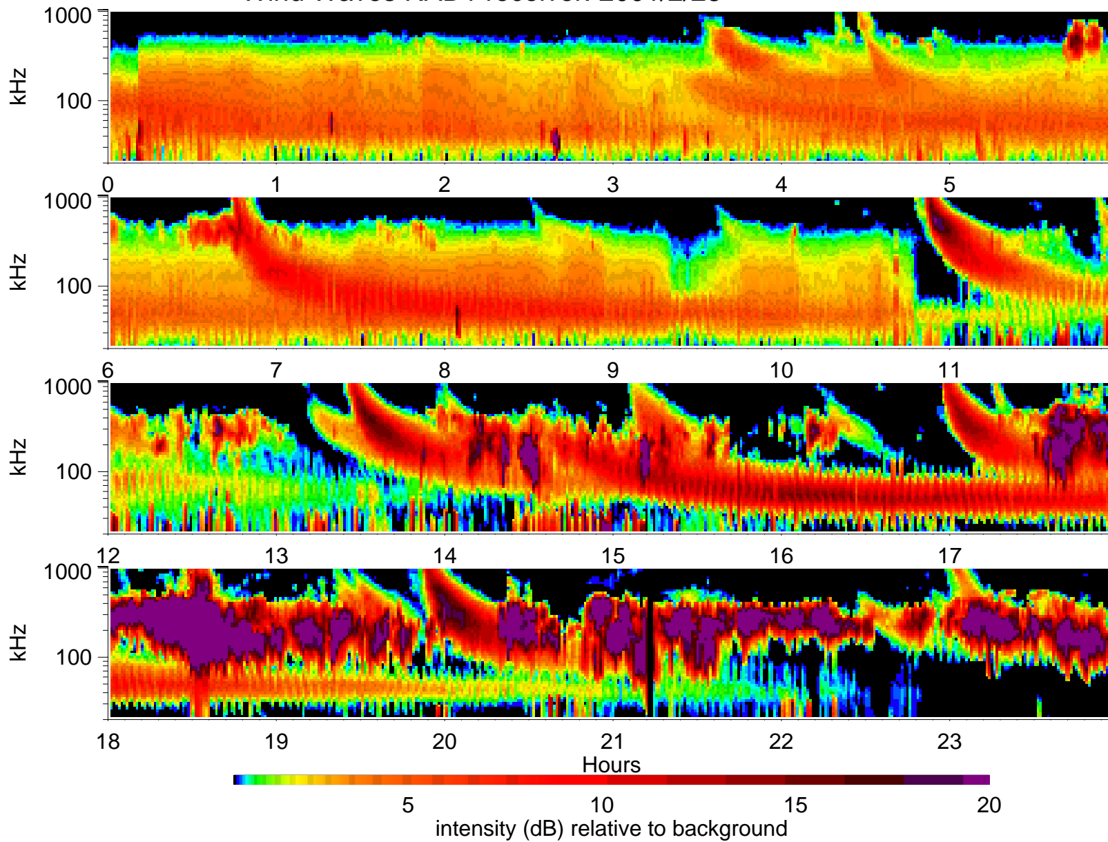
Wind Waves RAD1 receiver: 2001/2/28
