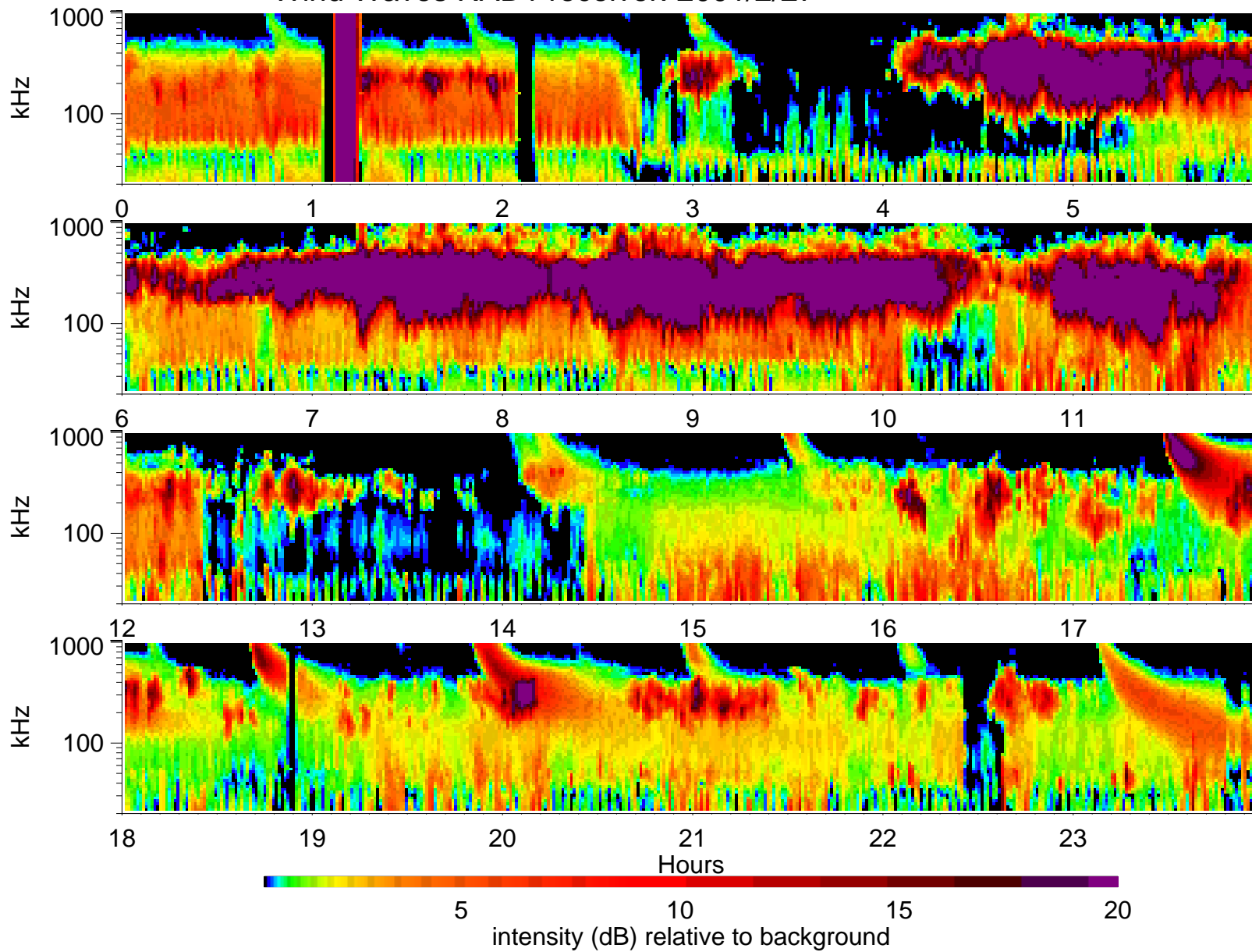
Wind Waves RAD1 receiver: 2001/2/27
