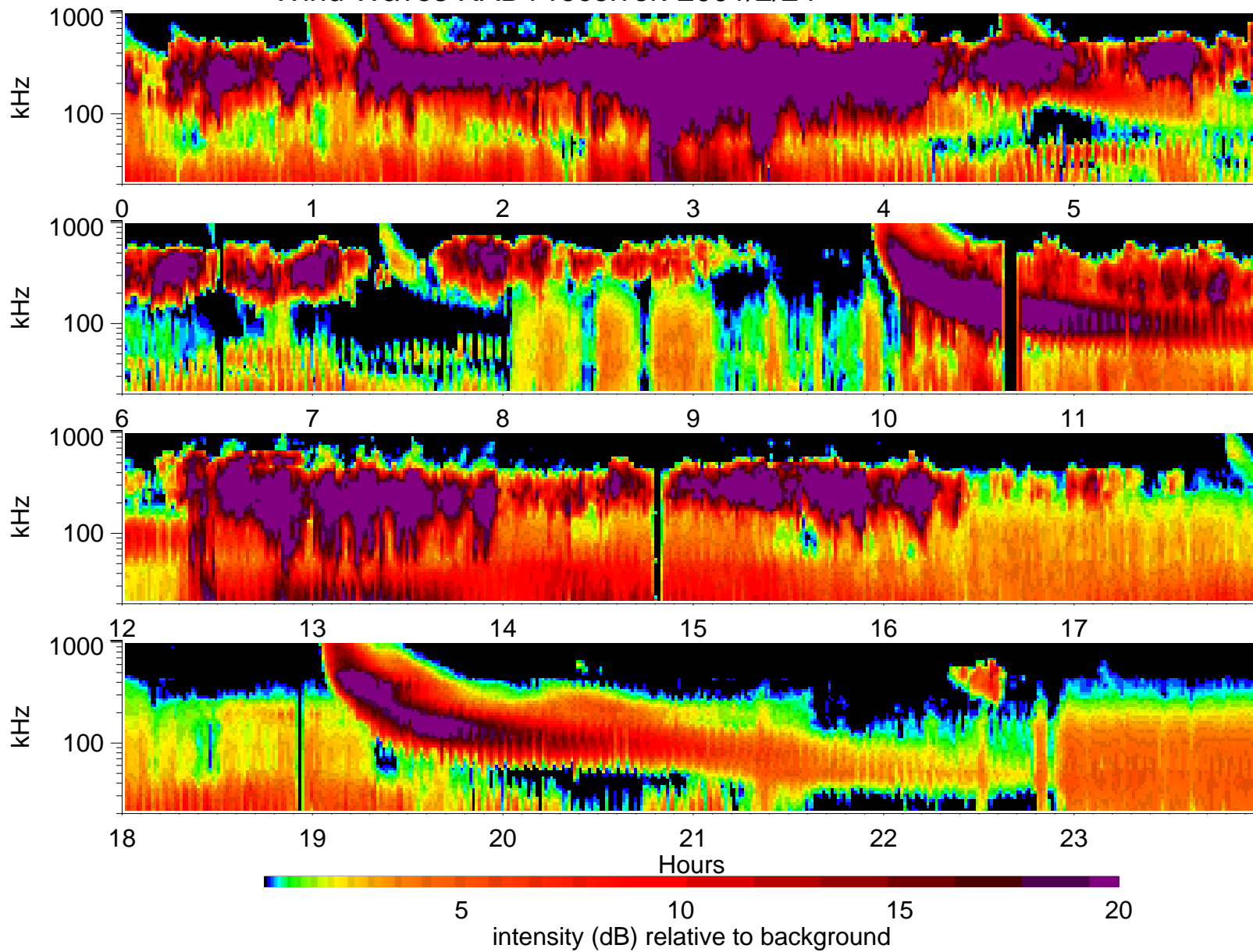
Wind Waves RAD1 receiver: 2001/2/24
