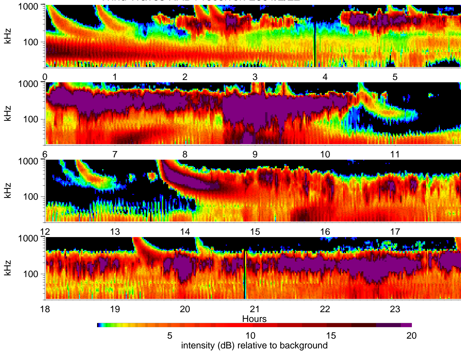
Wind Waves RAD1 receiver: 2001/2/22
