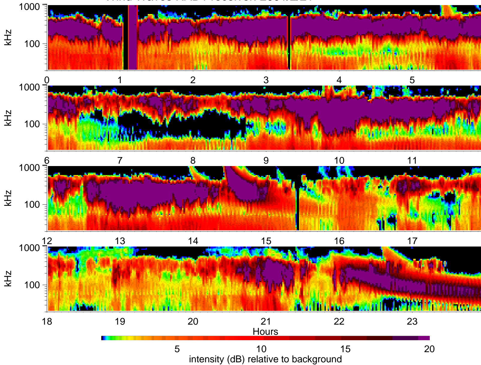
Wind Waves RAD1 receiver: 2001/2/21
