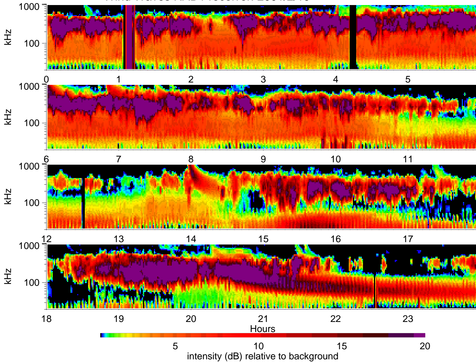
Wind Waves RAD1 receiver: 2001/2/19
