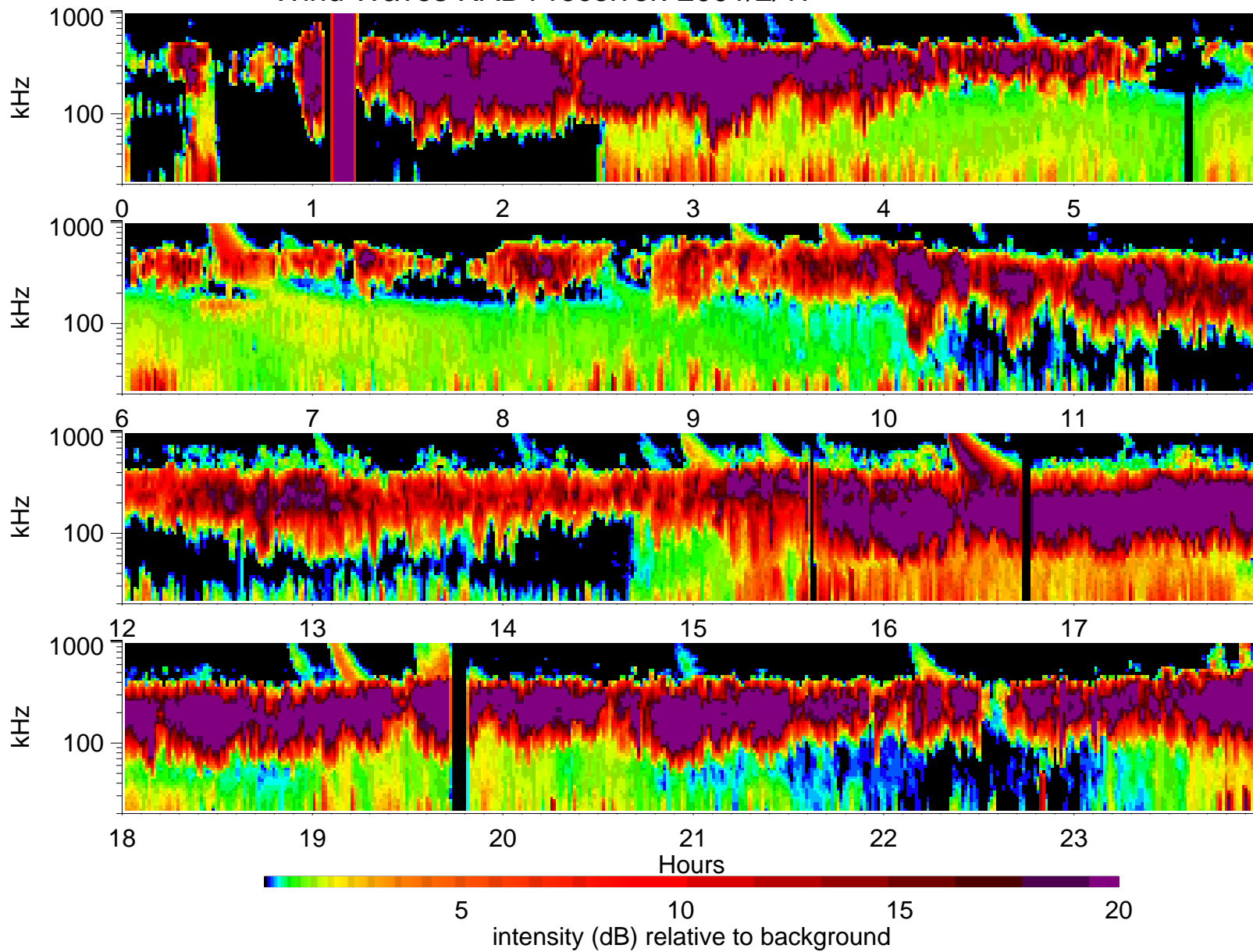
Wind Waves RAD1 receiver: 2001/2/17
