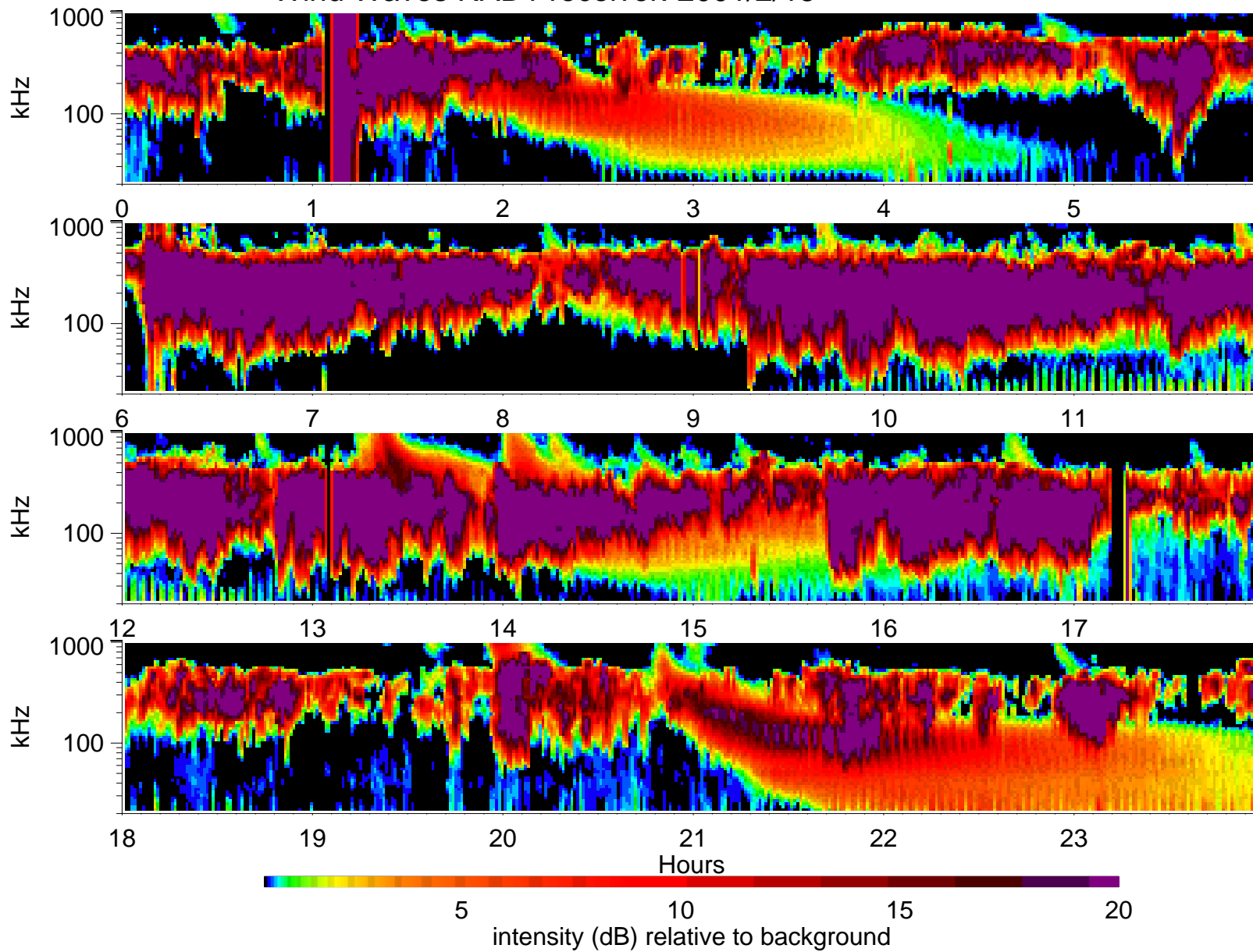
Wind Waves RAD1 receiver: 2001/2/15
