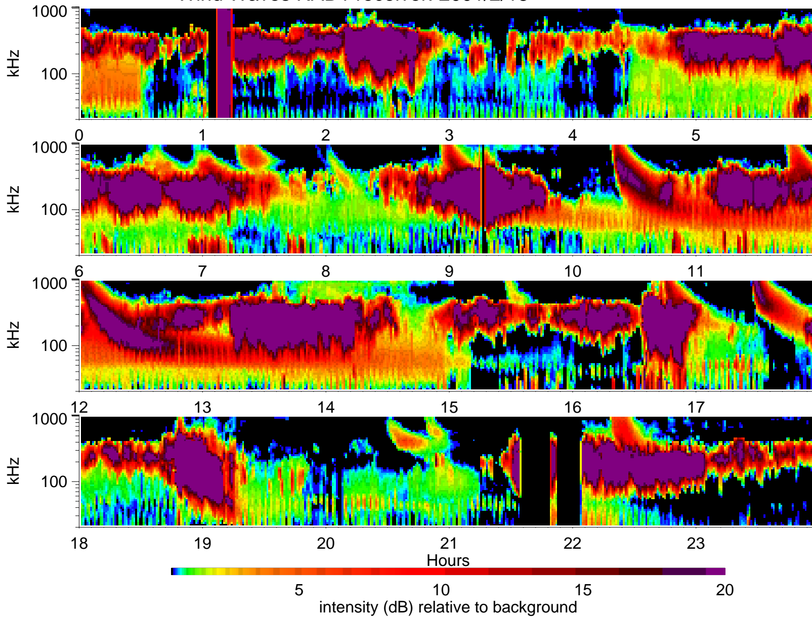
Wind Waves RAD1 receiver: 2001/2/13
