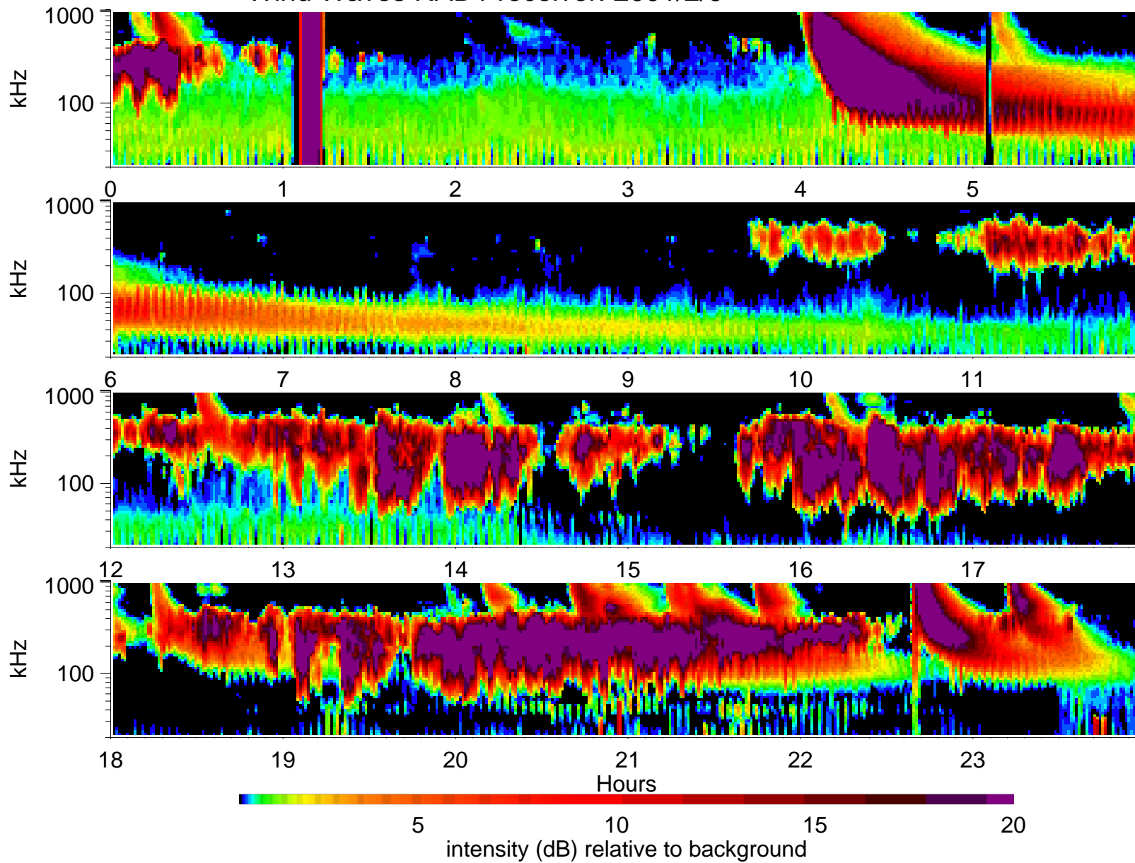
Wind Waves RAD1 receiver: 2001/2/9
