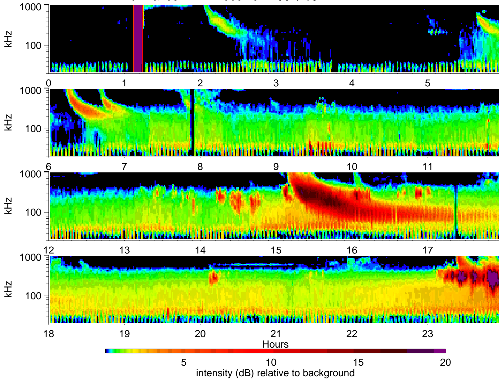
Wind Waves RAD1 receiver: 2001/2/5
