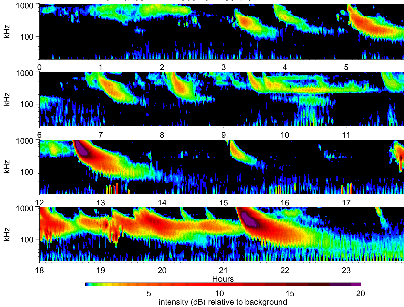
Wind Waves RAD1 receiver: 2001/2/4
