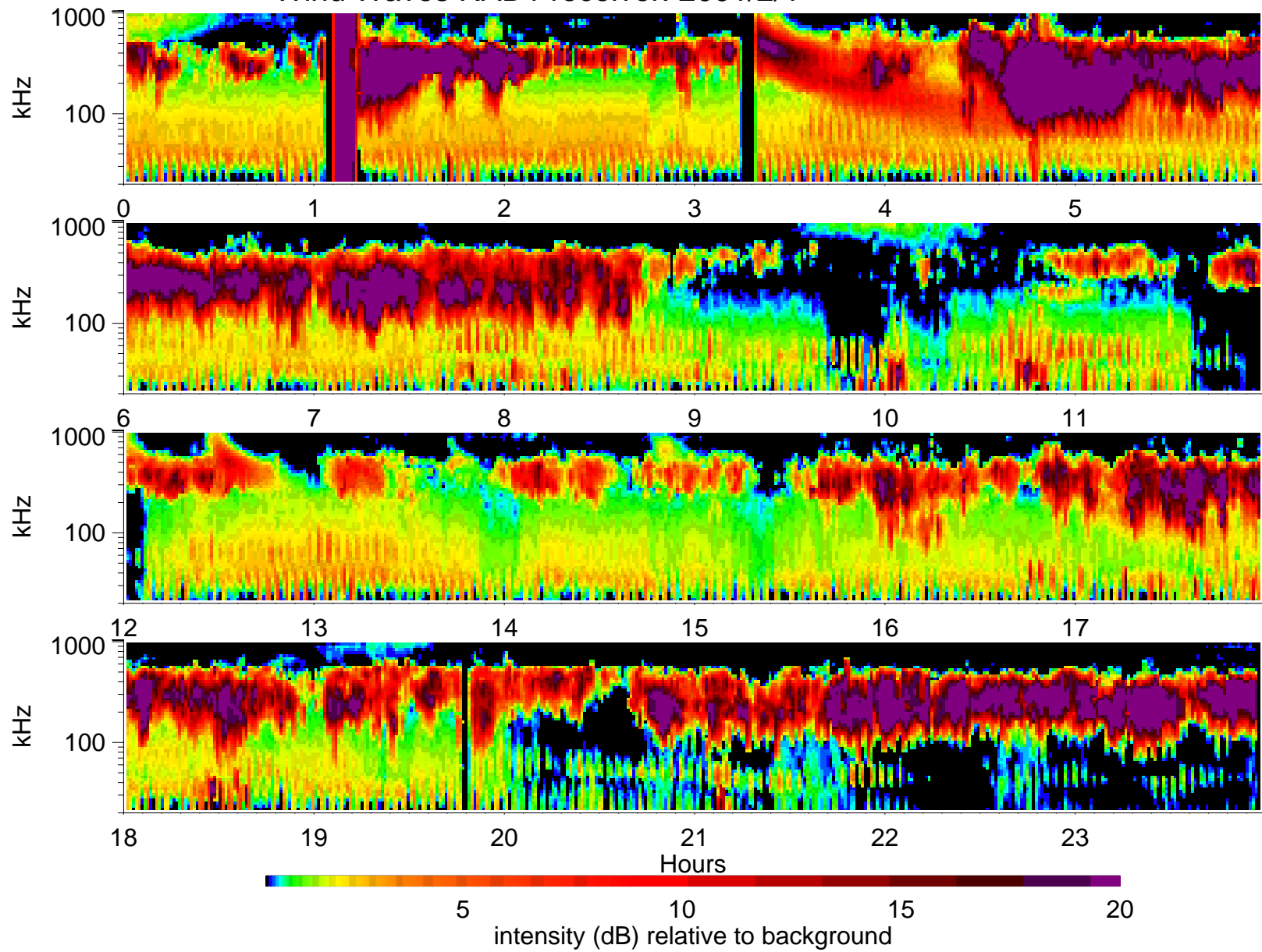
Wind Waves RAD1 receiver: 2001/2/1
