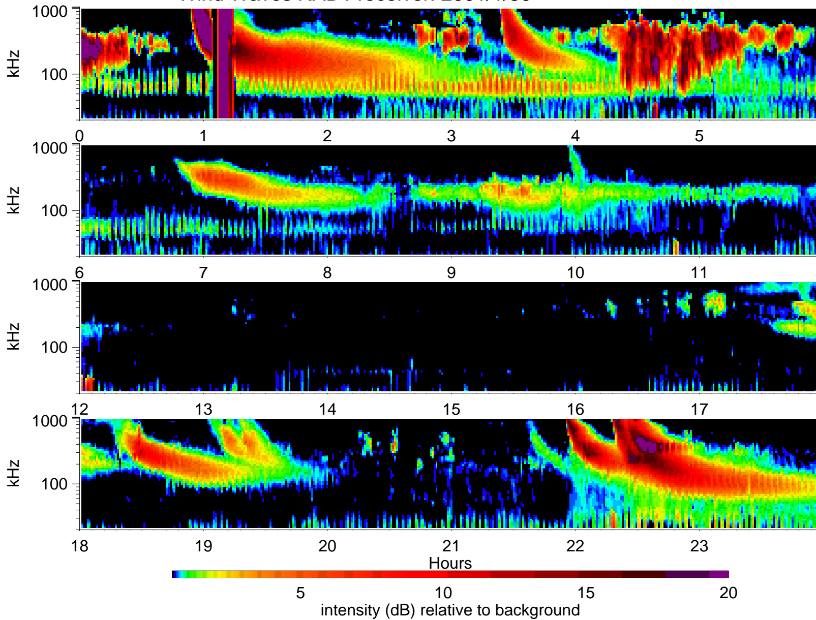
Wind Waves RAD1 receiver: 2001/1/30
