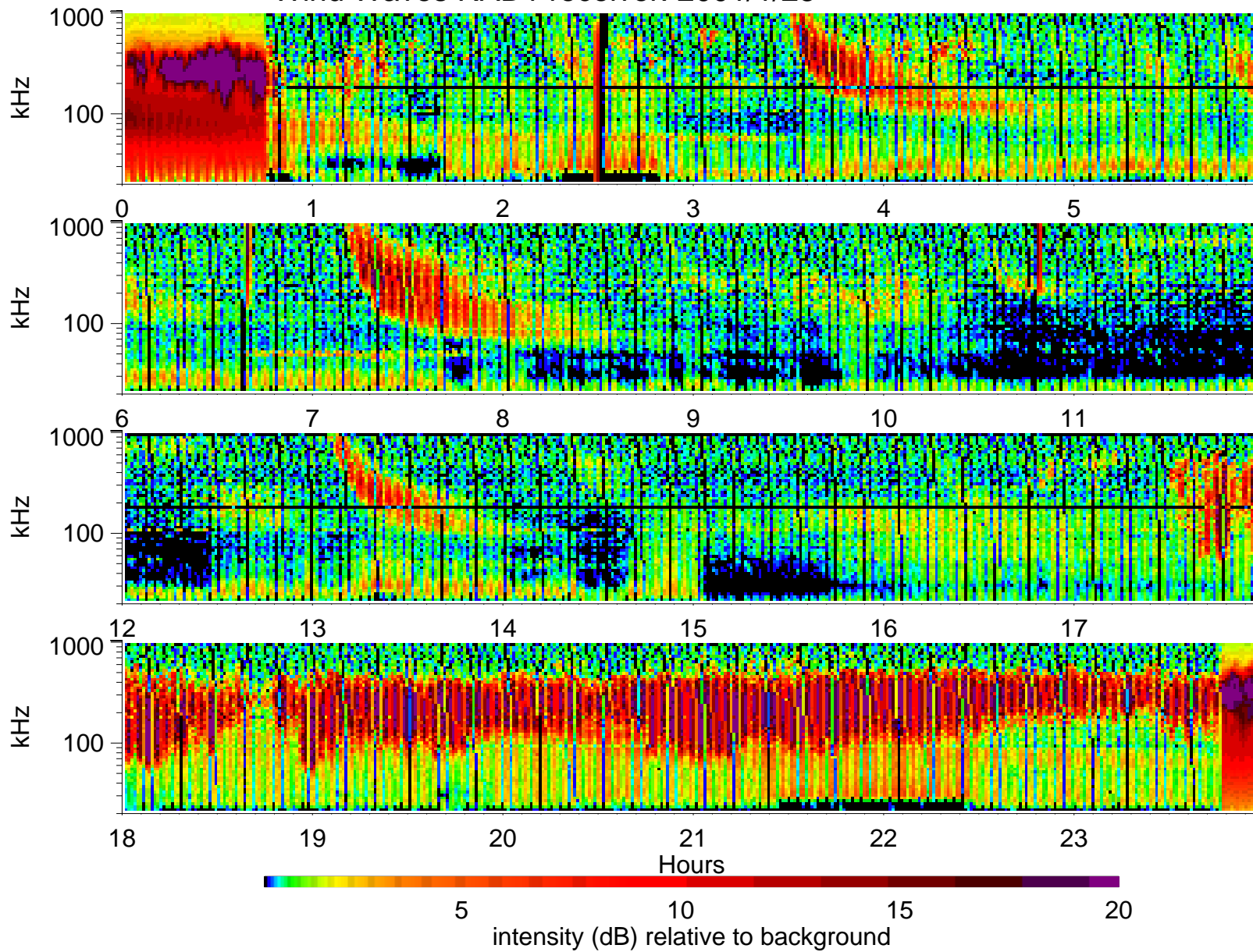
Wind Waves RAD1 receiver: 2001/1/25
