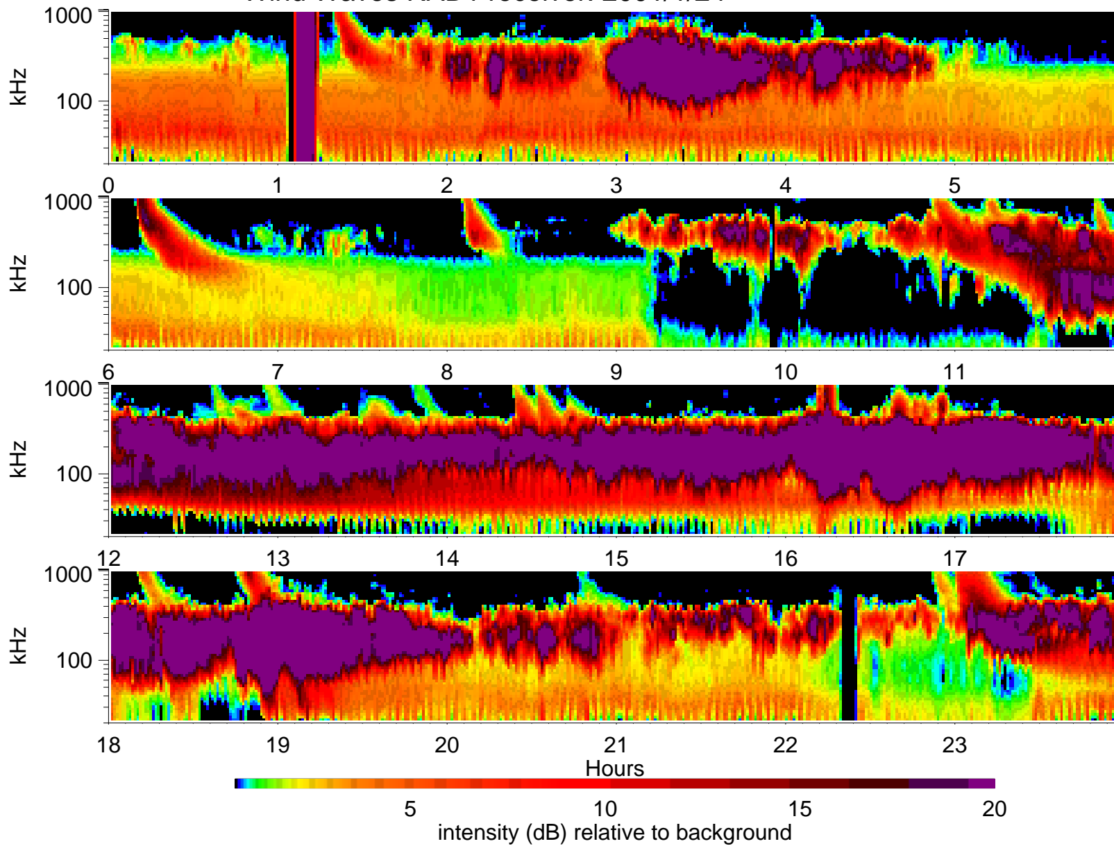
Wind Waves RAD1 receiver: 2001/1/24
