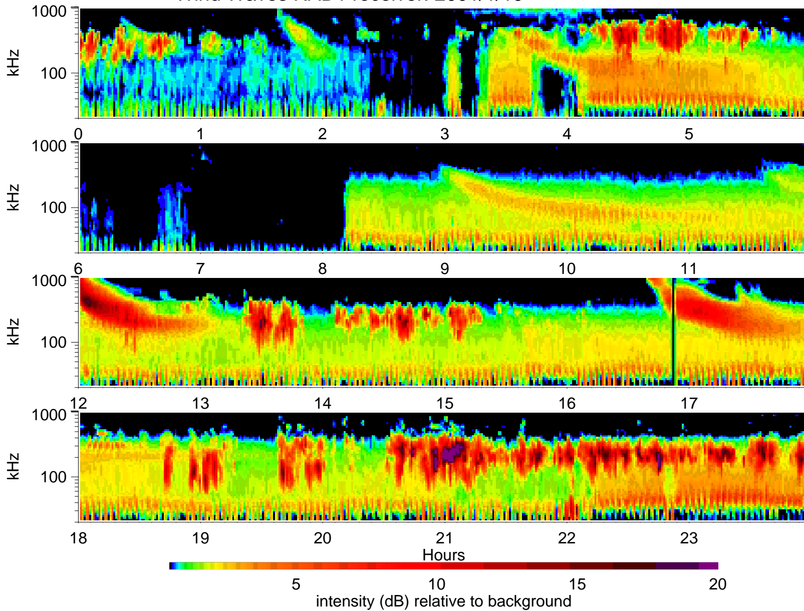
Wind Waves RAD1 receiver: 2001/1/19
