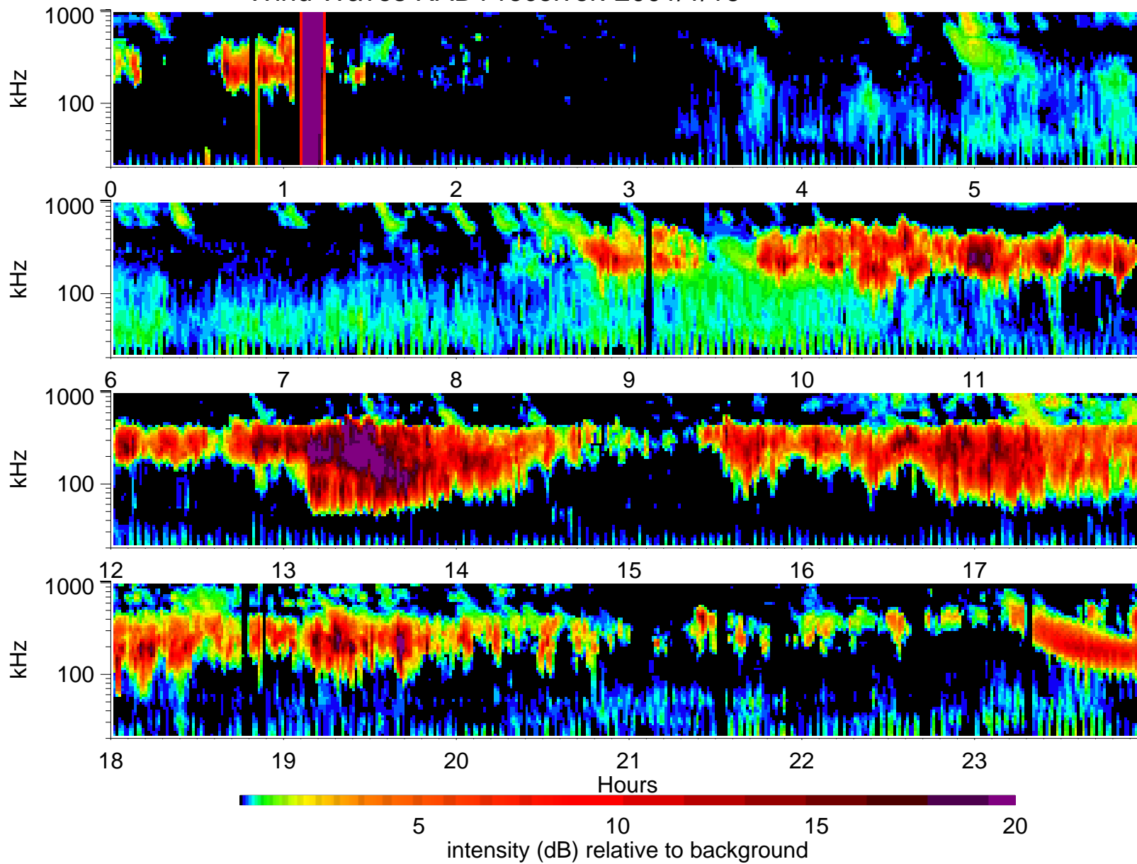
Wind Waves RAD1 receiver: 2001/1/16
