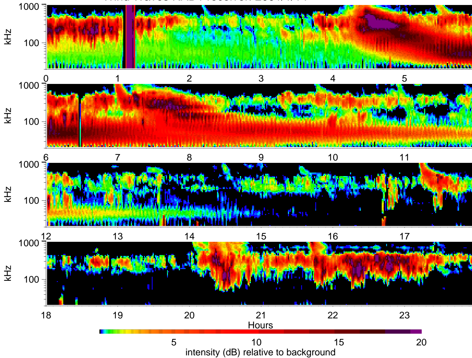
Wind Waves RAD1 receiver: 2001/1/14
