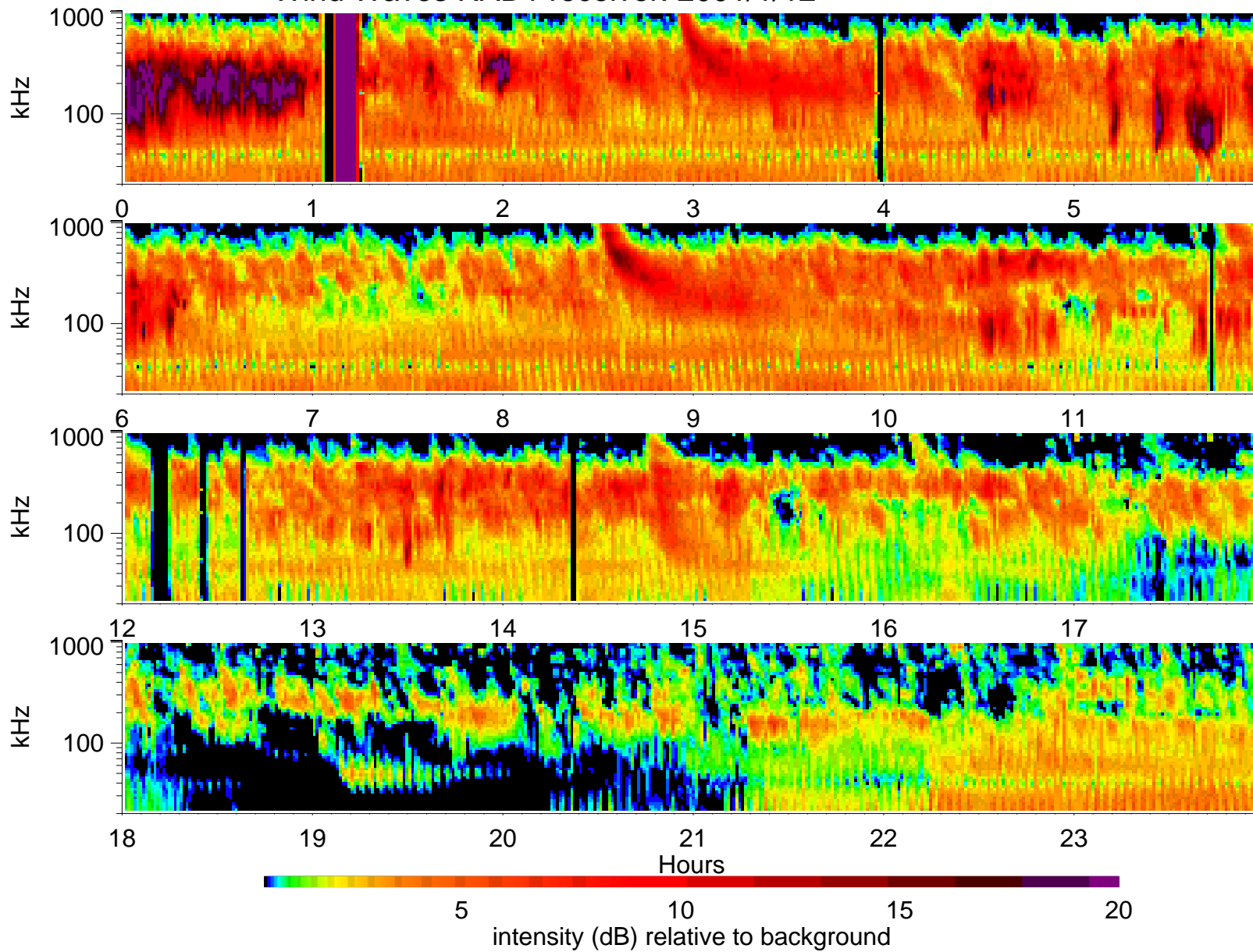
Wind Waves RAD1 receiver: 2001/1/12
