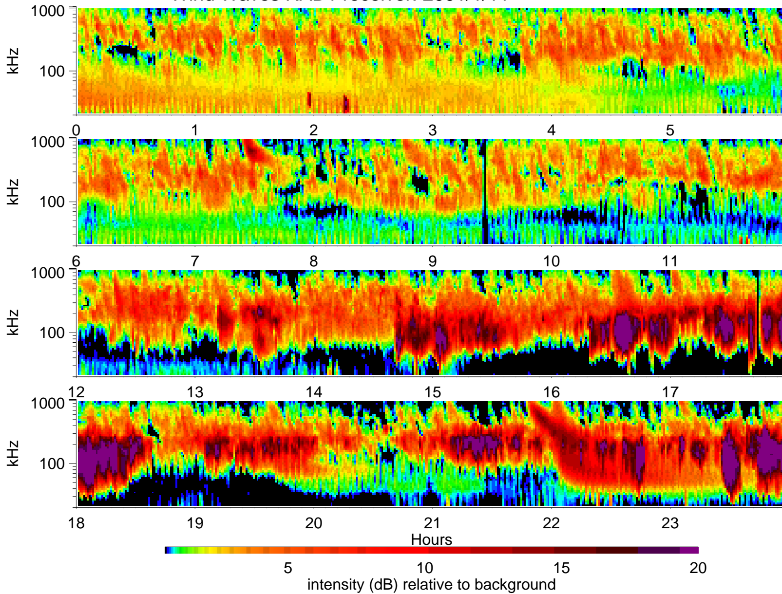
Wind Waves RAD1 receiver: 2001/1/11
