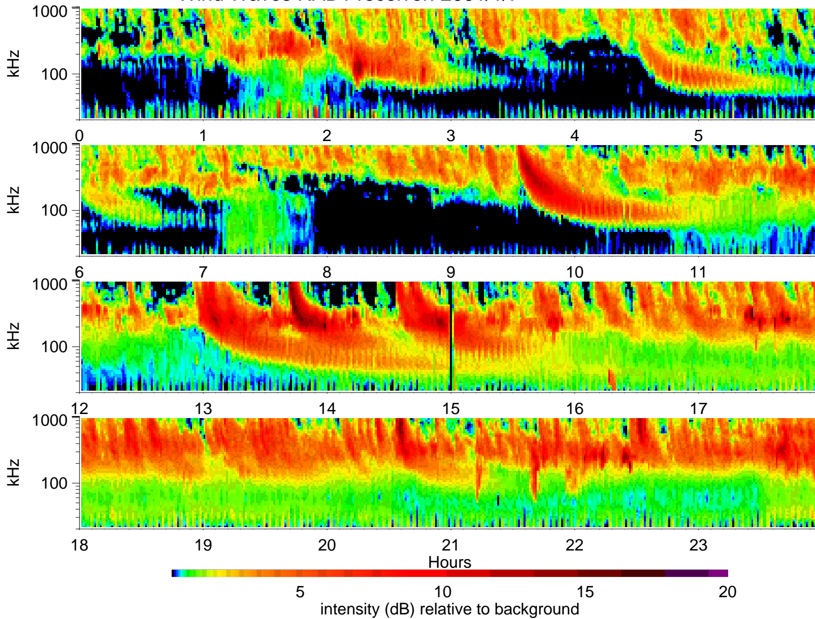
Wind Waves RAD1 receiver: 2001/1/7
