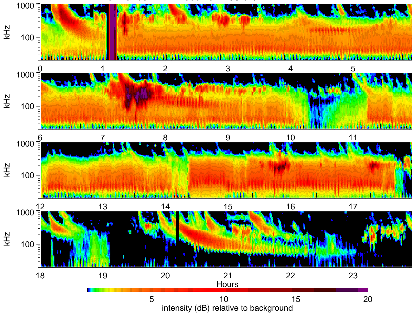
Wind Waves RAD1 receiver: 2001/1/4
