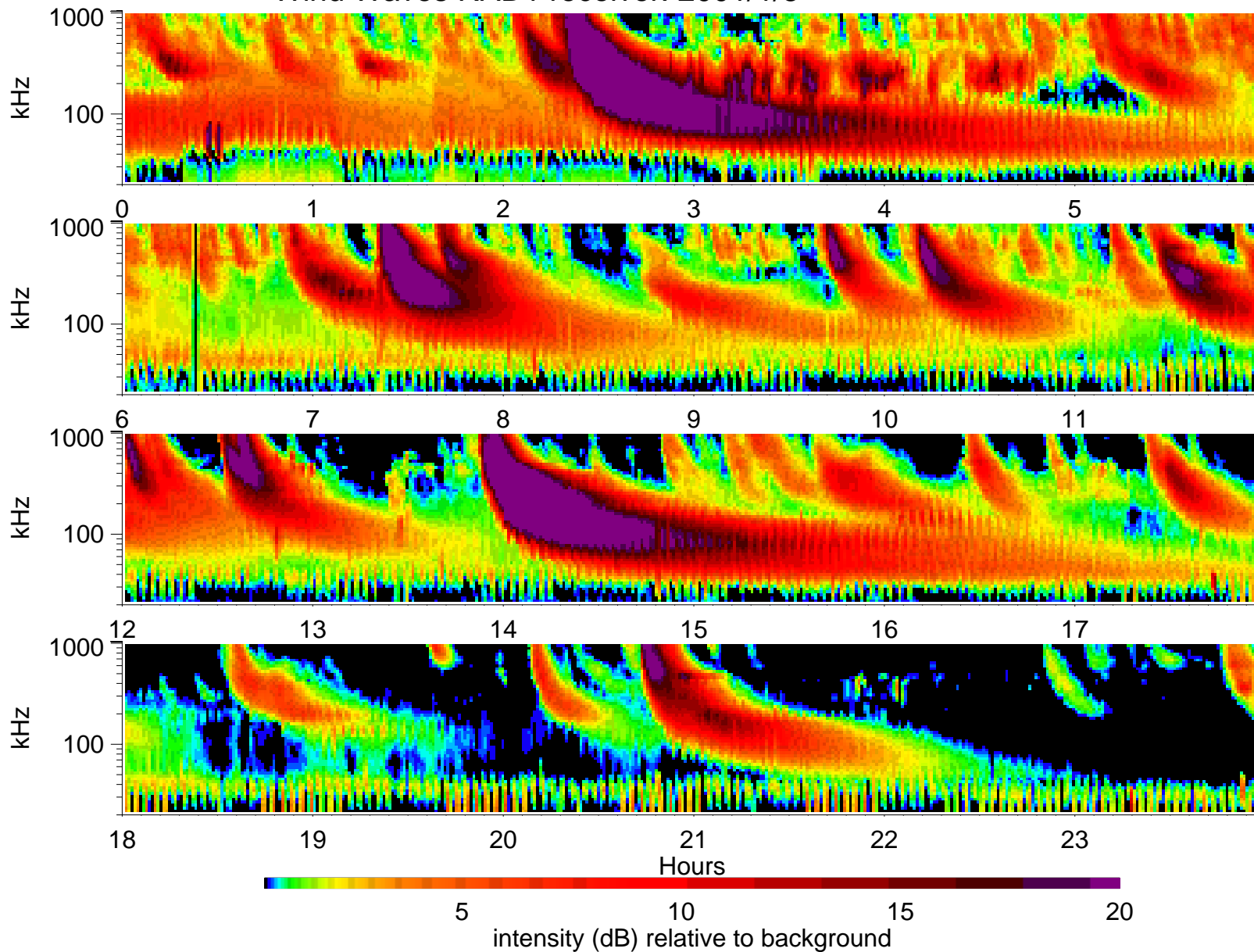
Wind Waves RAD1 receiver: 2001/1/3
