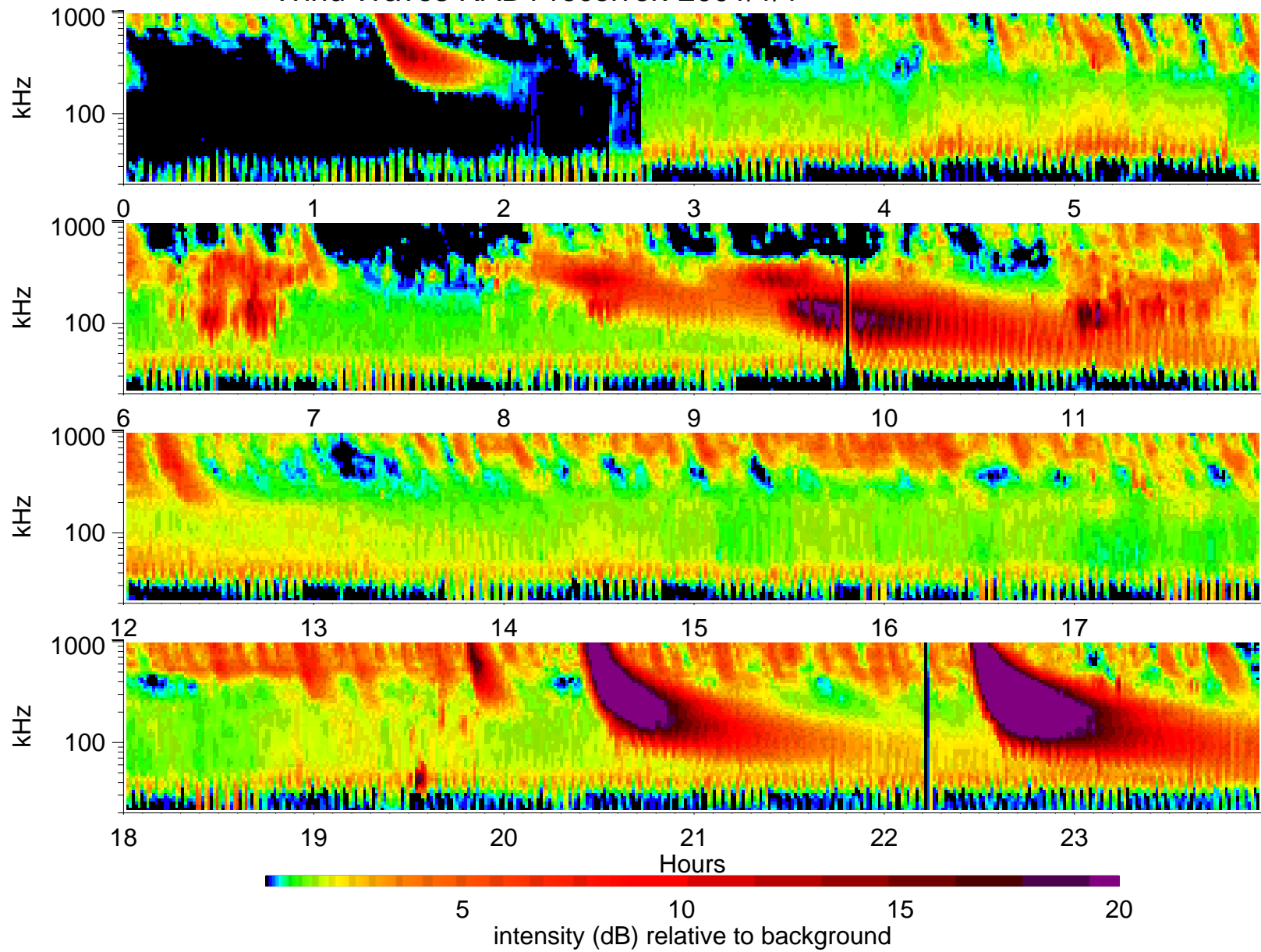
Wind Waves RAD1 receiver: 2001/1/1
