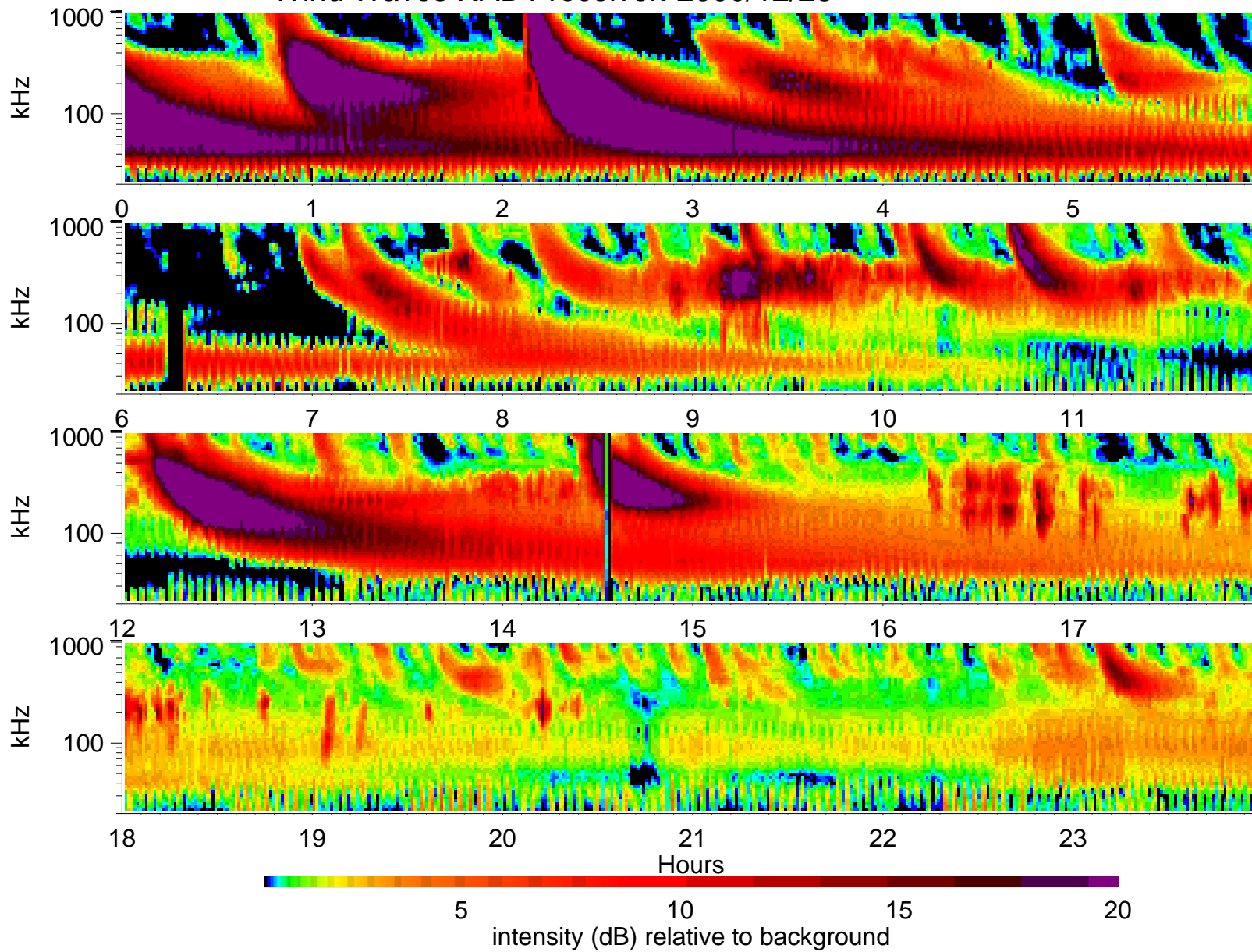
Wind Waves RAD1 receiver: 2000/12/28
