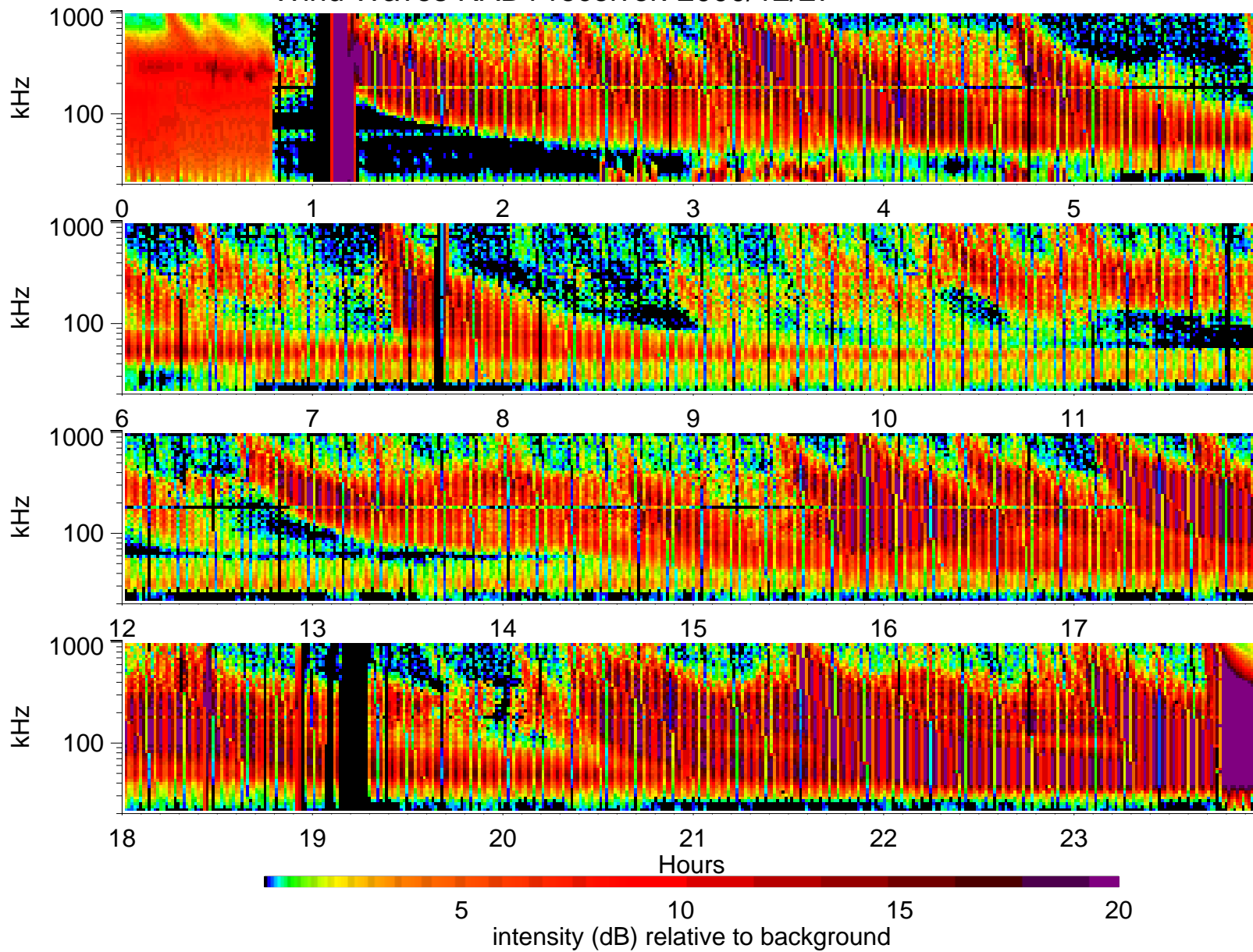
Wind Waves RAD1 receiver: 2000/12/27
