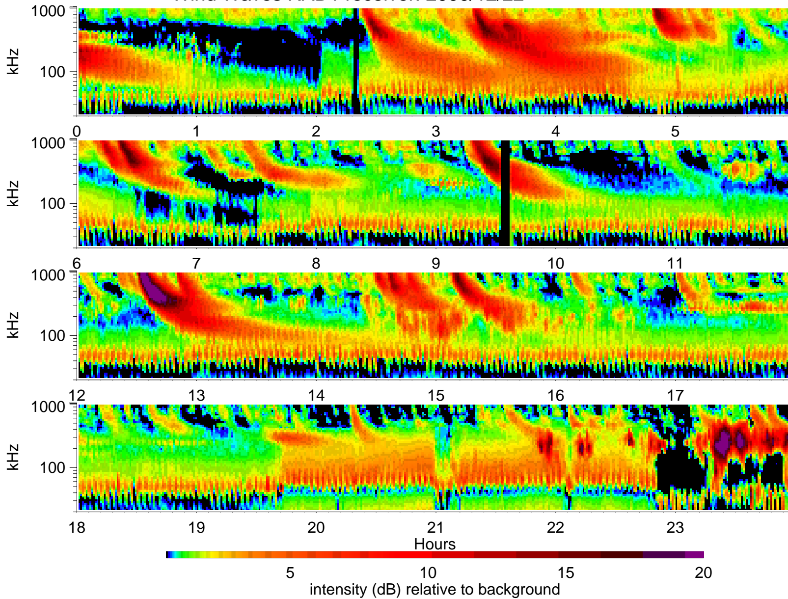
Wind Waves RAD1 receiver: 2000/12/22
