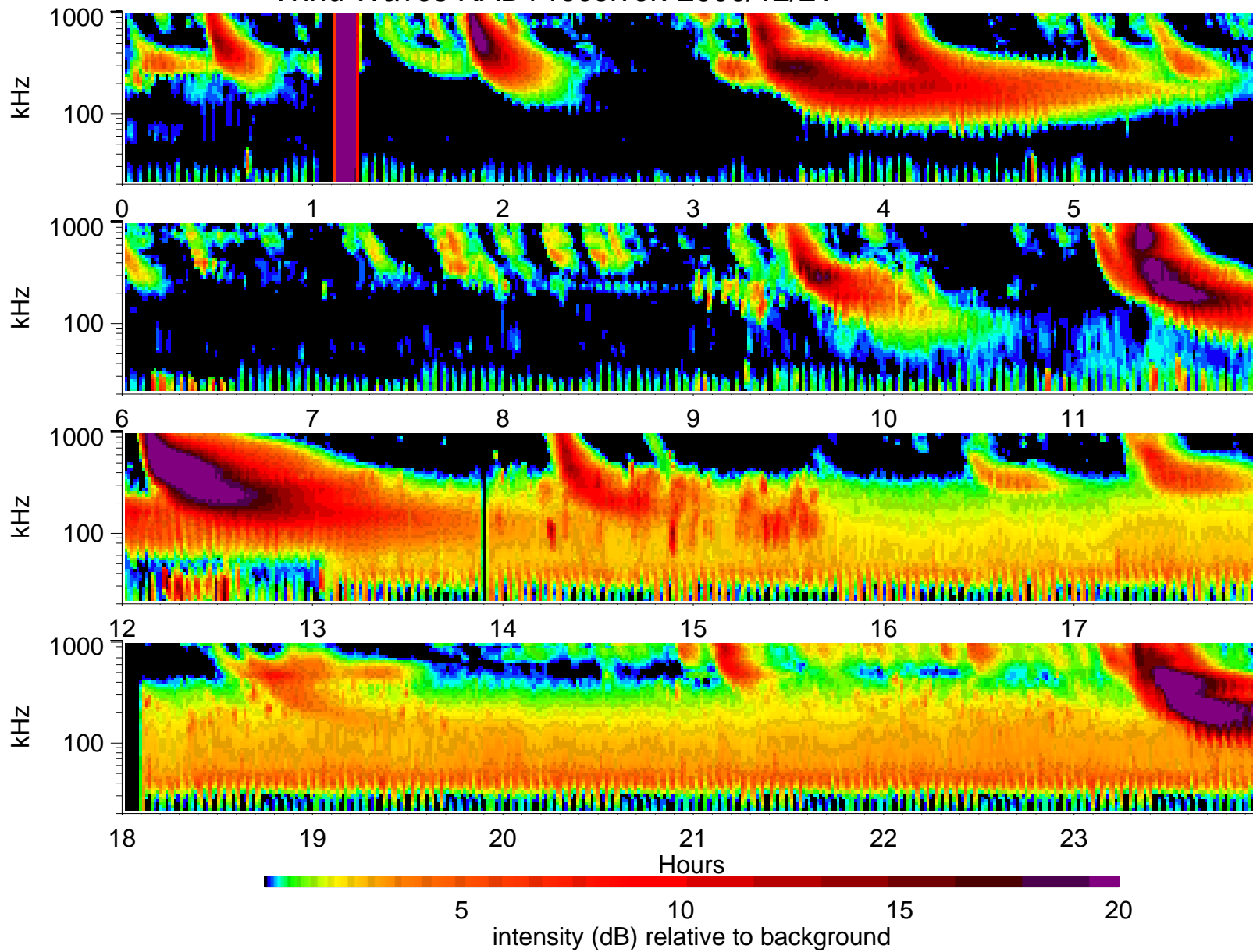
Wind Waves RAD1 receiver: 2000/12/21
