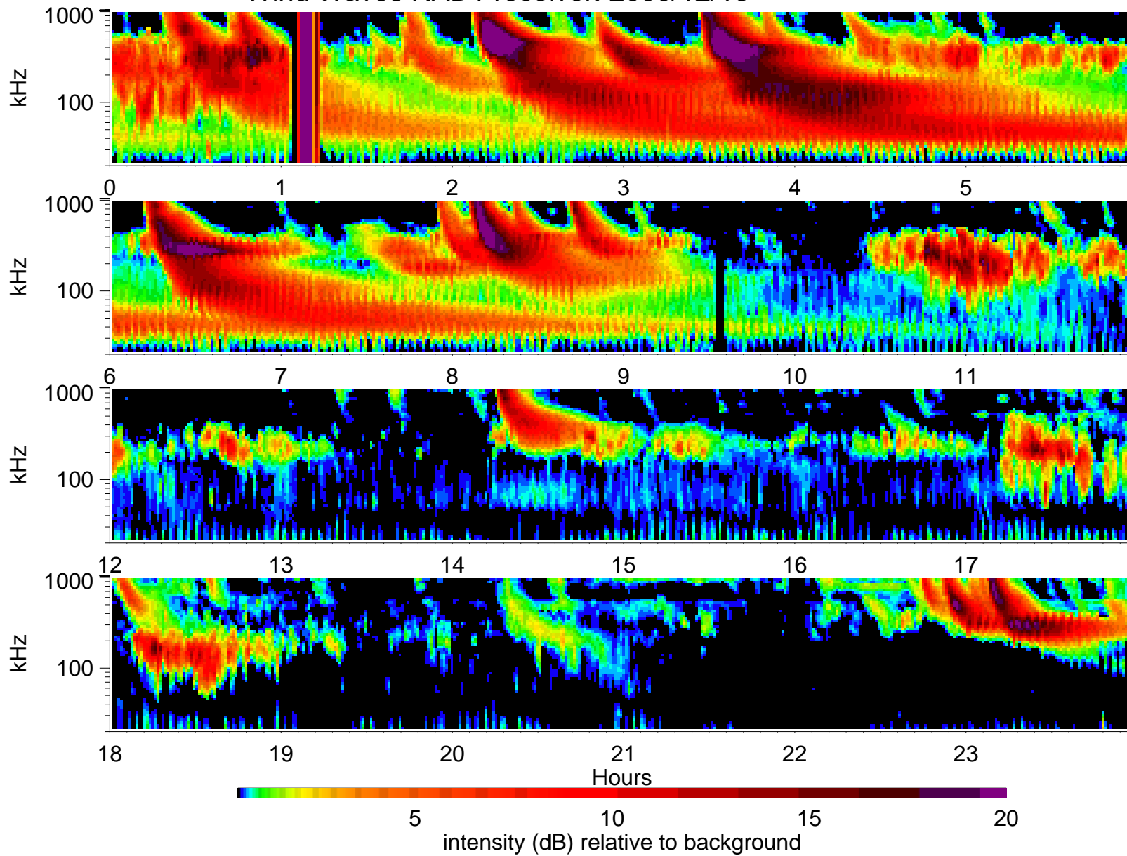
Wind Waves RAD1 receiver: 2000/12/19
