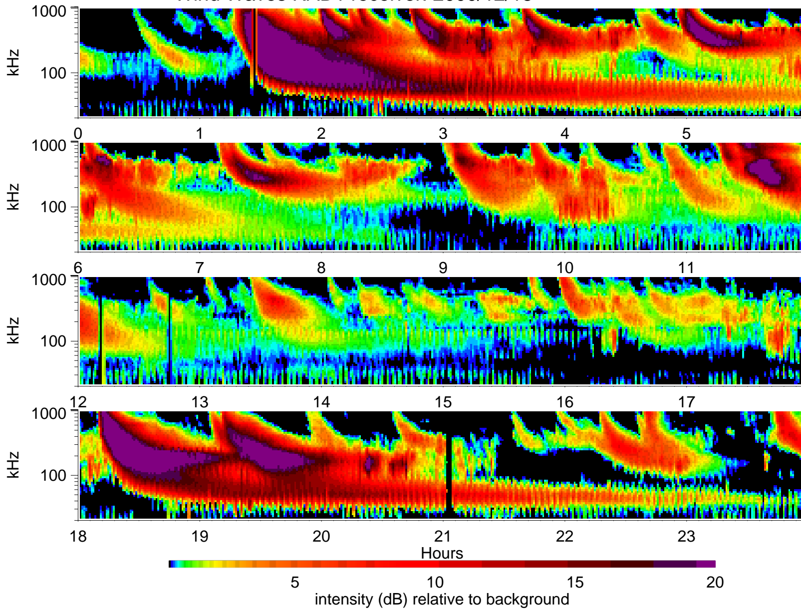
Wind Waves RAD1 receiver: 2000/12/18
