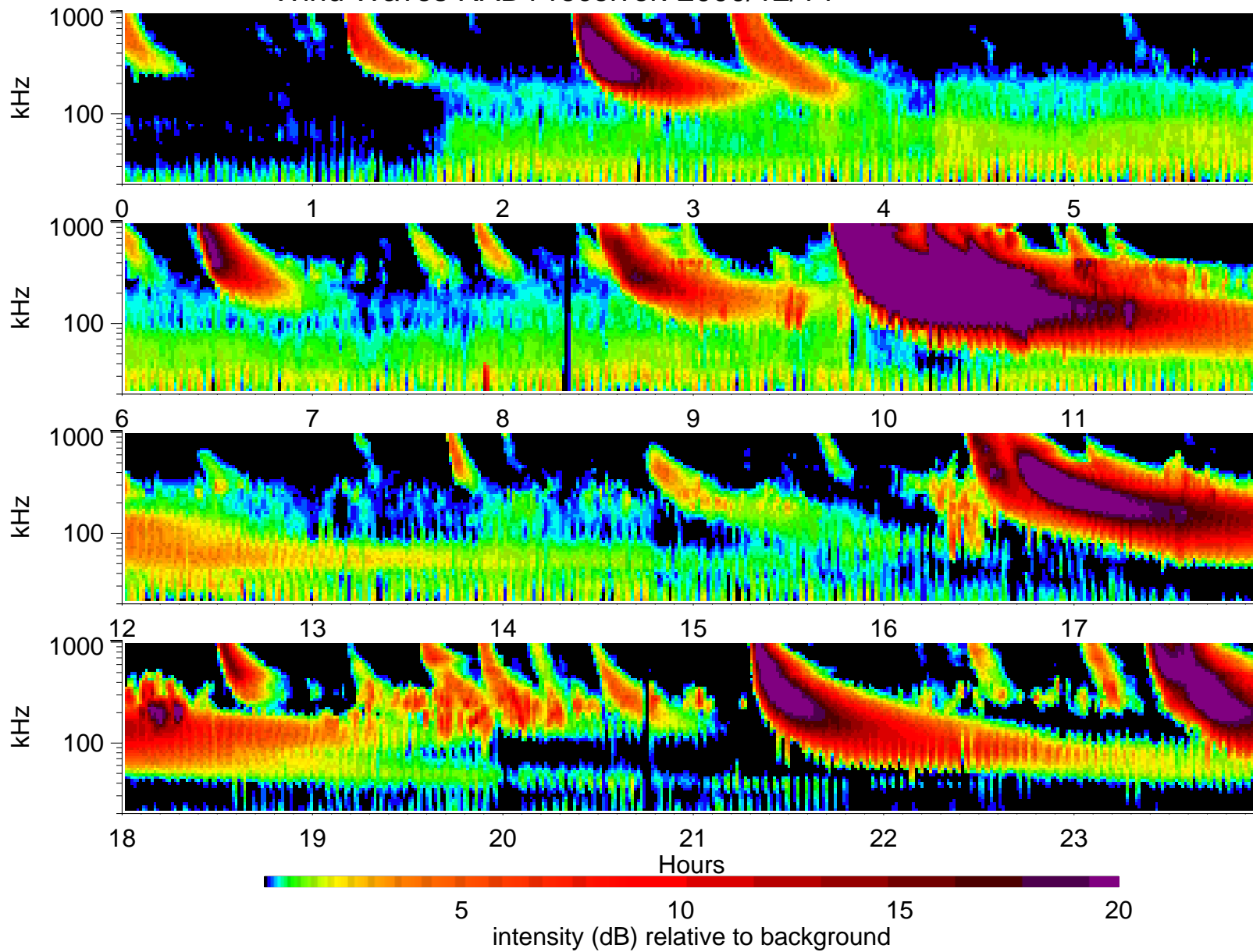
Wind Waves RAD1 receiver: 2000/12/14
