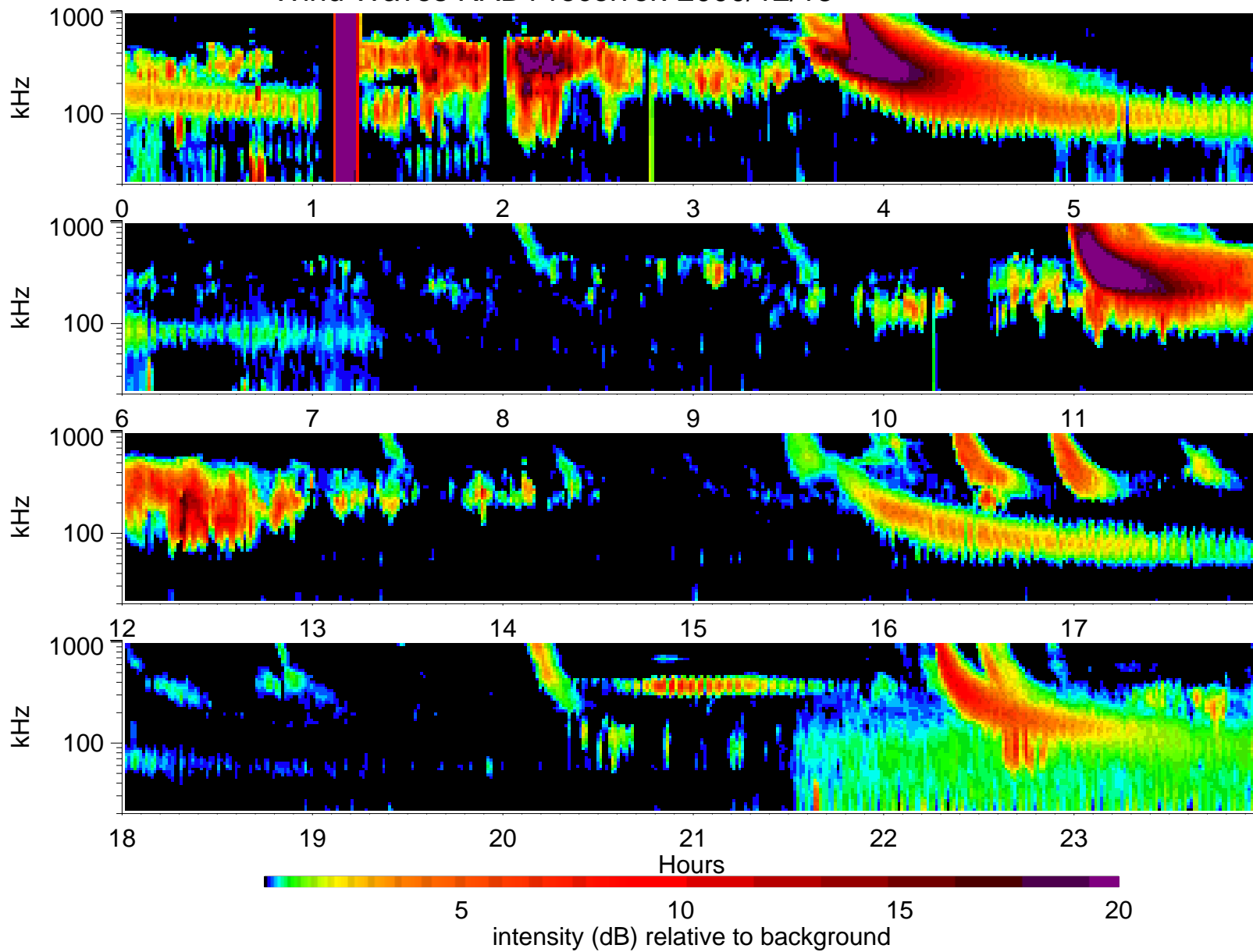
Wind Waves RAD1 receiver: 2000/12/13
