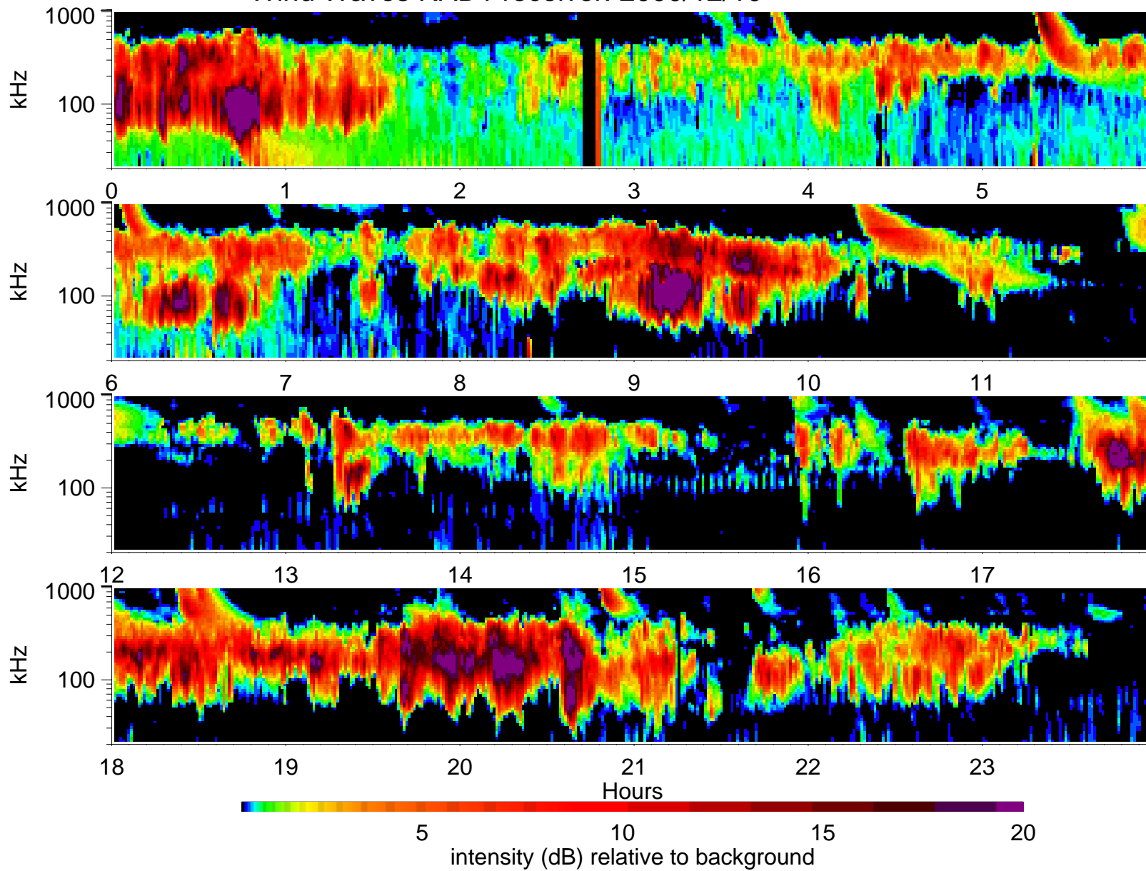
Wind Waves RAD1 receiver: 2000/12/10
