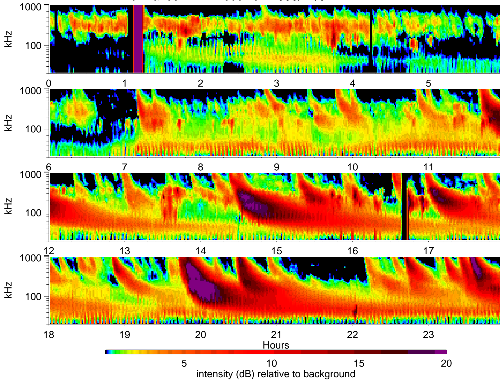
Wind Waves RAD1 receiver: 2000/12/5
