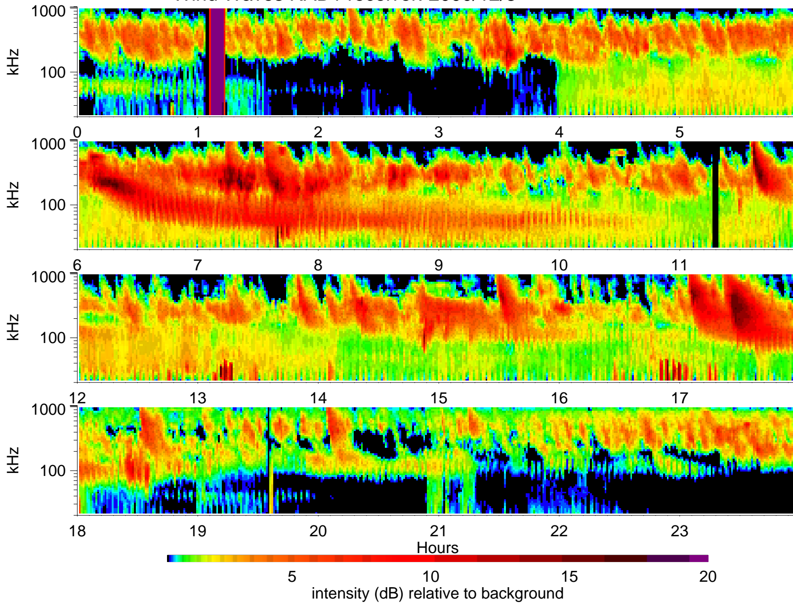
Wind Waves RAD1 receiver: 2000/12/3
