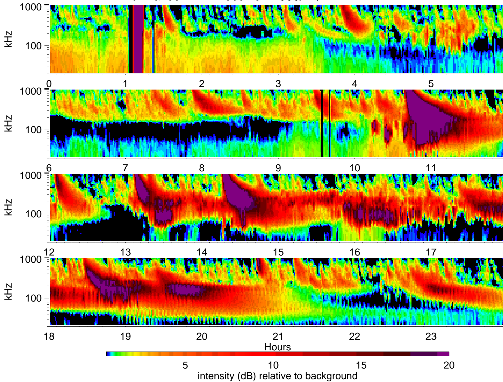
Wind Waves RAD1 receiver: 2000/12/1
