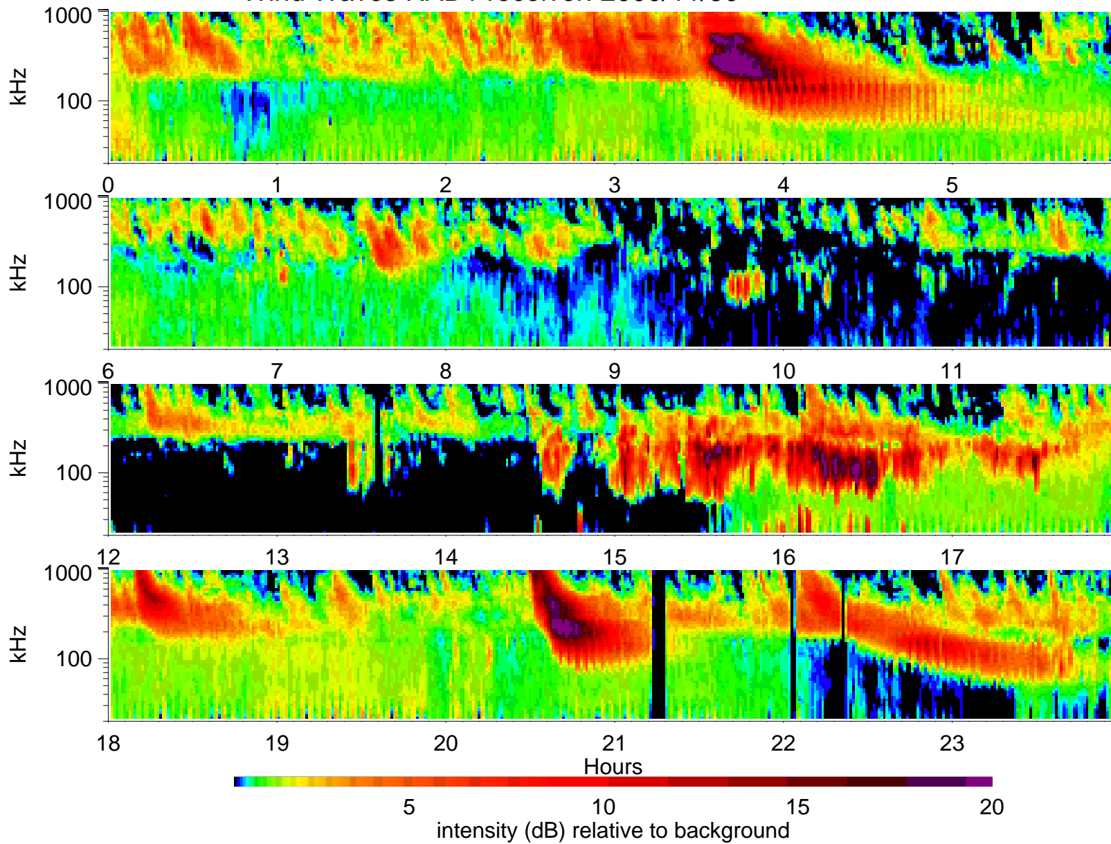
Wind Waves RAD1 receiver: 2000/11/30
