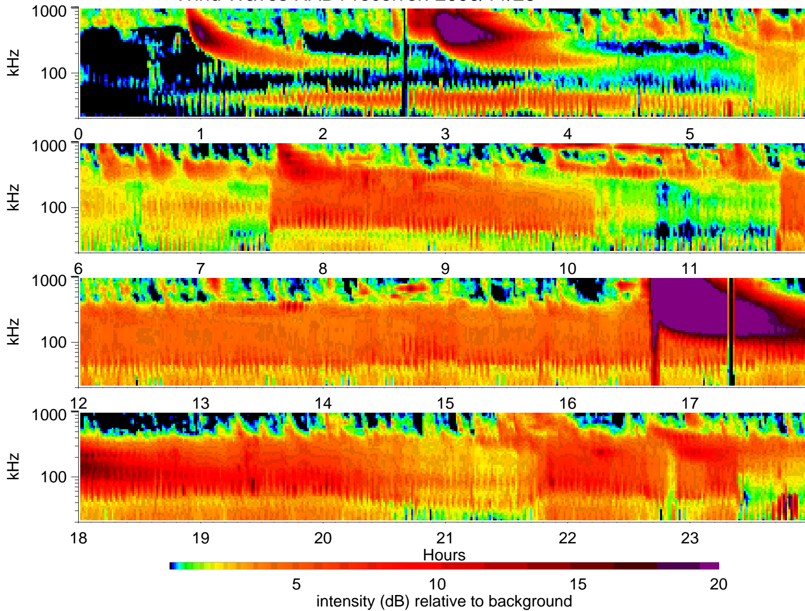
Wind Waves RAD1 receiver: 2000/11/26
