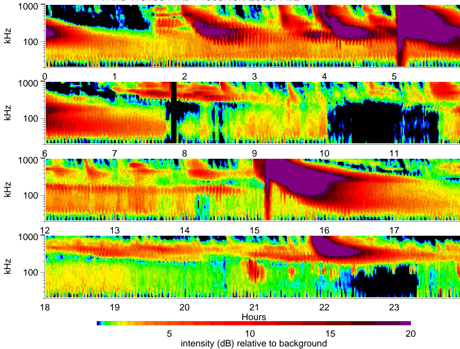
Wind Waves RAD1 receiver: 2000/11/24
