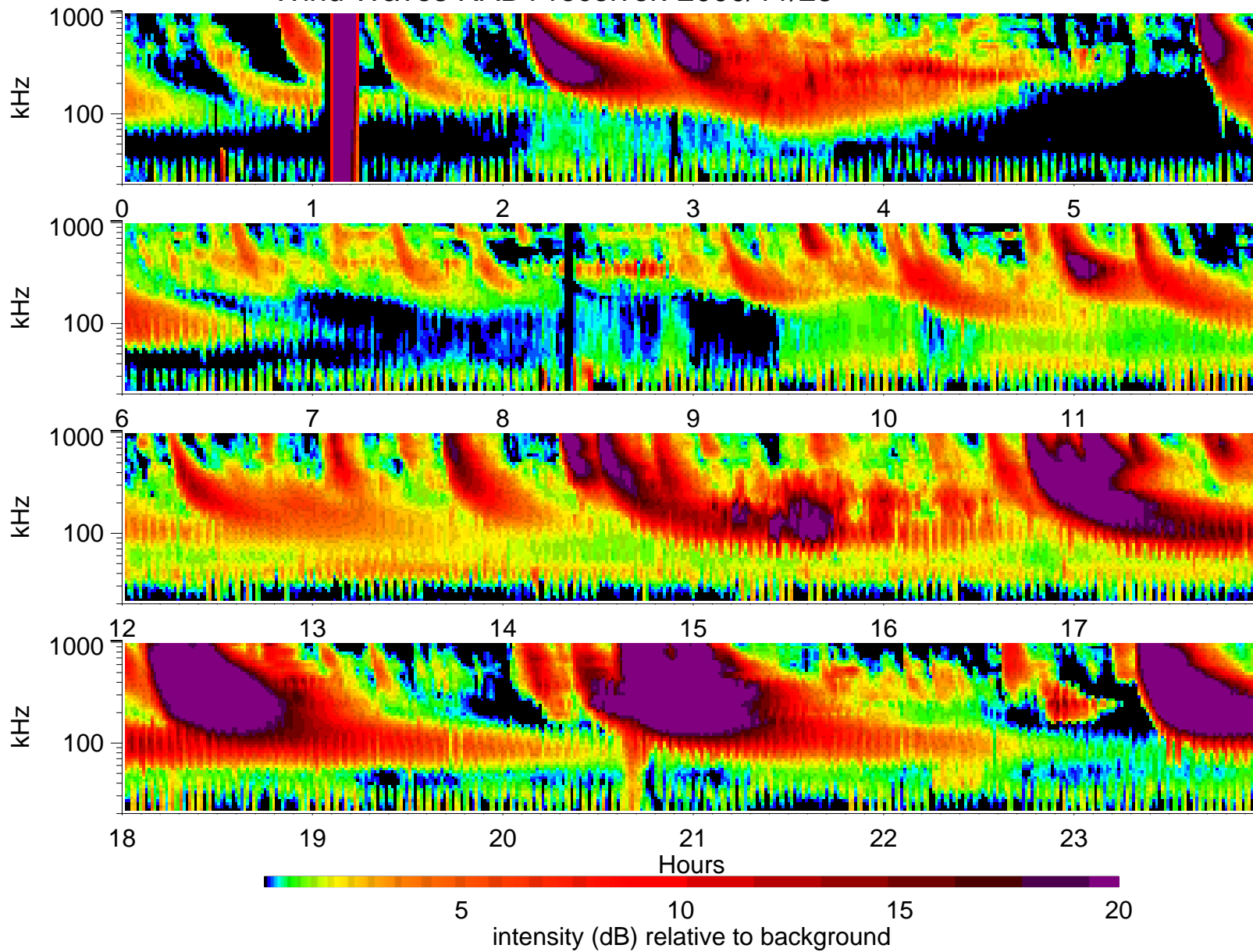
Wind Waves RAD1 receiver: 2000/11/23
