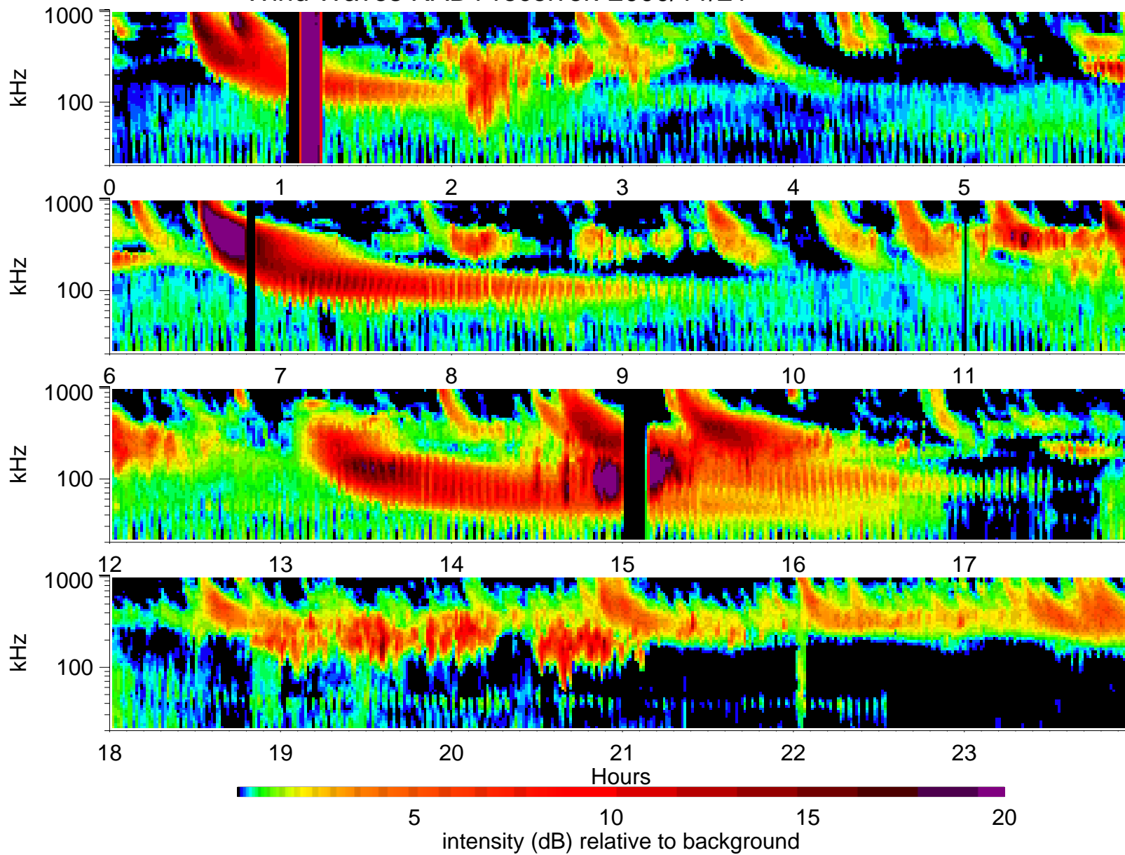
Wind Waves RAD1 receiver: 2000/11/21
