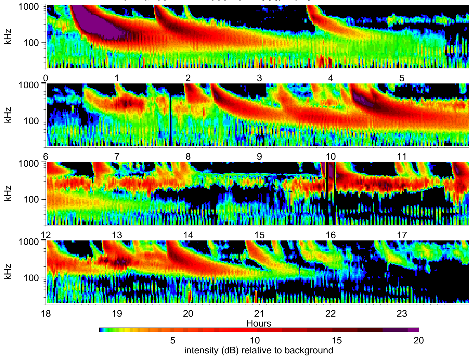
Wind Waves RAD1 receiver: 2000/11/20
